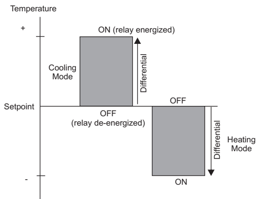
Figure 2: Operation of relay in according to Setpoint and Differential Settings for both Heating and Cooling Mode
